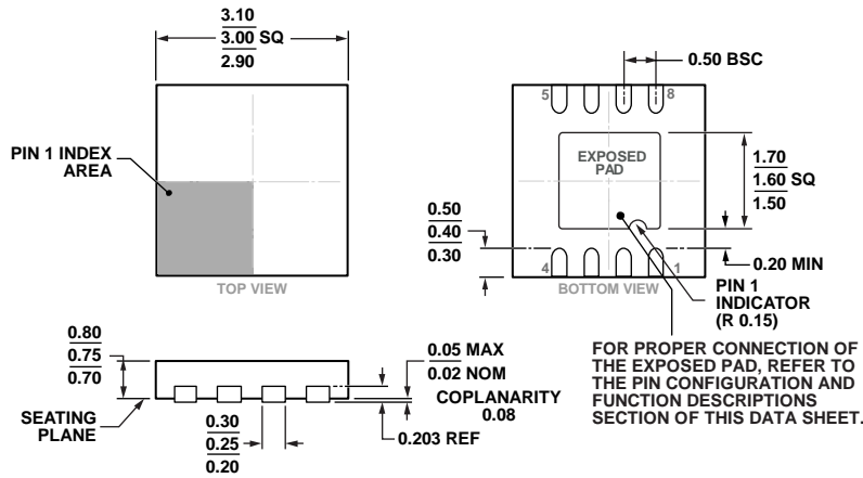
Figure 115. 8-Lead Lead Frame Chip Scale Package [LFCSF_WD]
