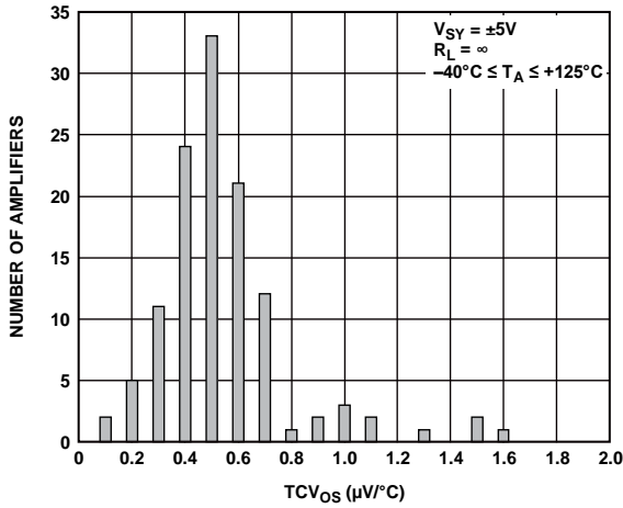
Figure 47. TCV OS Distribution, LFCSP
