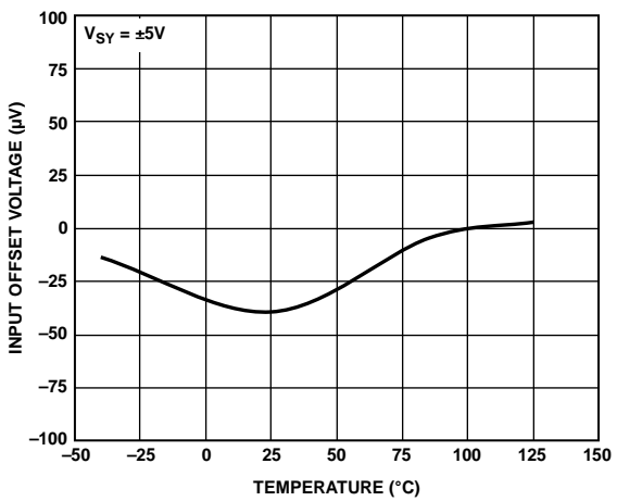
Figure 49. Input Offset Voltage vs. Temperature
