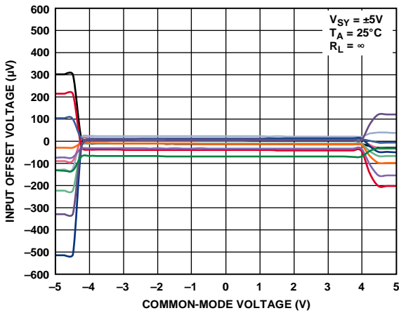
Figure 48. Input Offset Voltage vs. Common-Mode Voltage
